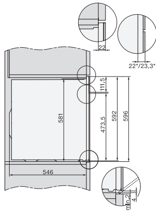
DO7860, Skizze
