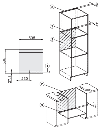
DO7860, Skizze
